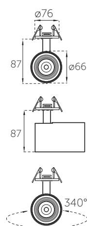
TRACK EMPOTRAR
