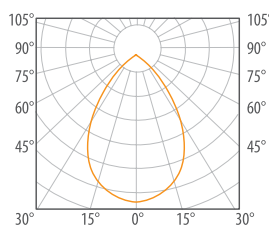
DIFUSOR FROSTED
