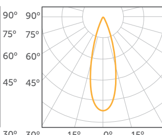
MEDIA 30°
