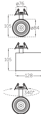
TRACK EMPOTRAR
